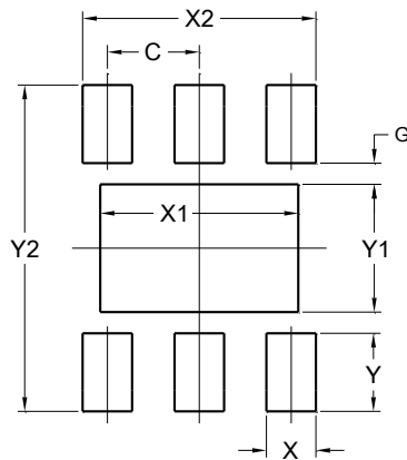
W-DFN2020-6 (Type SM)
