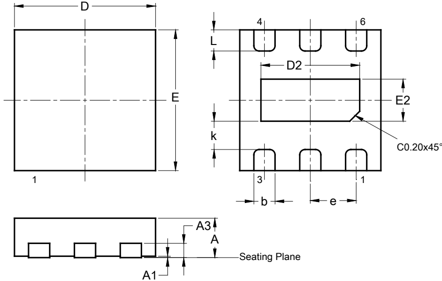
W-DFN2020-6 (Type A1)
