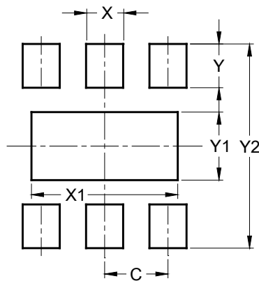
X2-DFN2020-6 (Type W)
