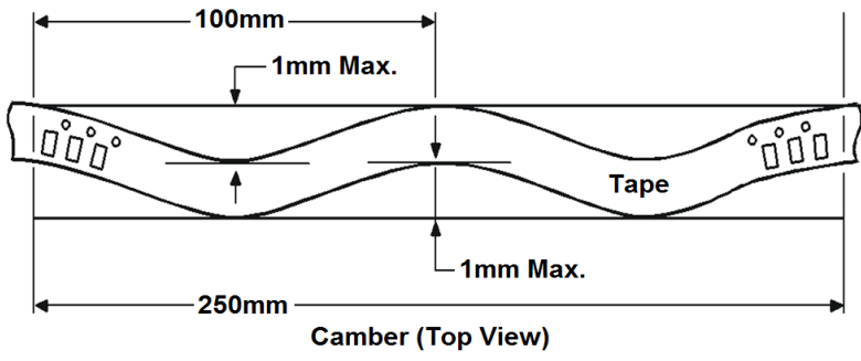
Allowable camber to be 1mm/100mm tape, non-cumulative
