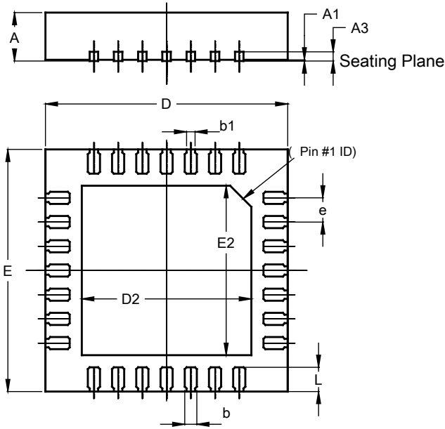
V-QFN4040-28 (Type TH)
