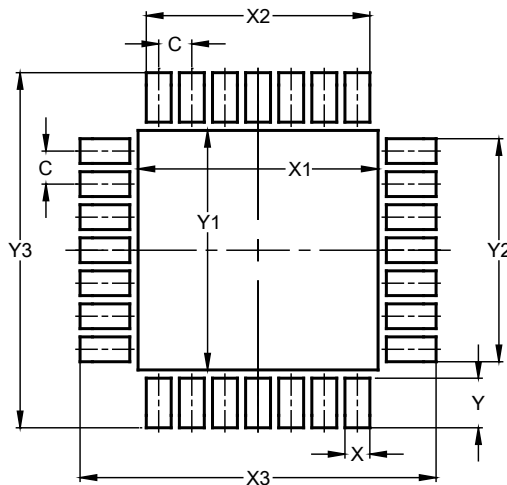
V-QFN4040-28 (Type TH)
