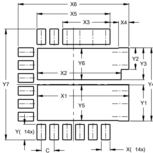
V-QFN4040-23
