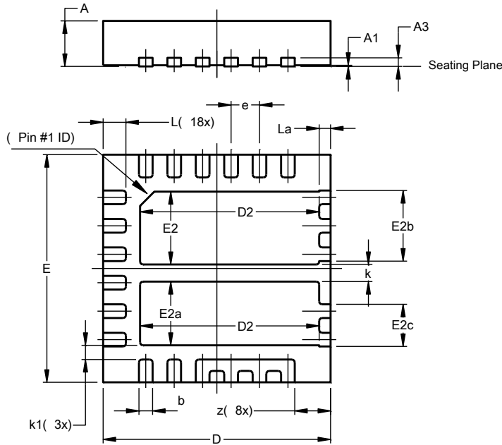
V-QFN4040-23
