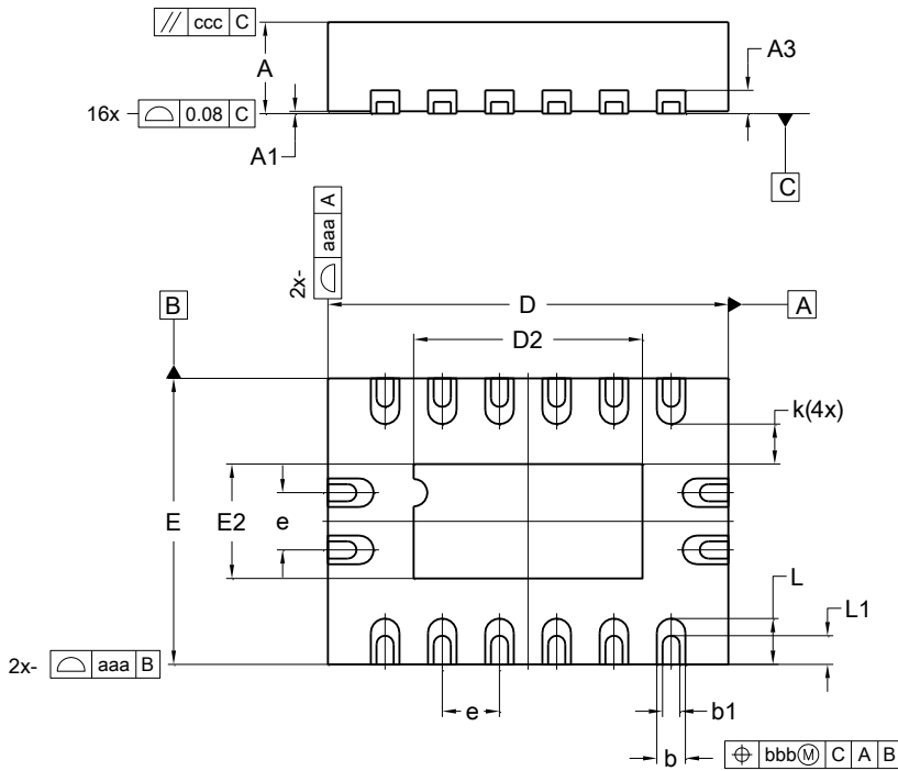
V-QFN3525-16/SWP (Type A)
