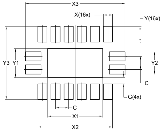
V-QFN3525-16/SWP (Type A)
