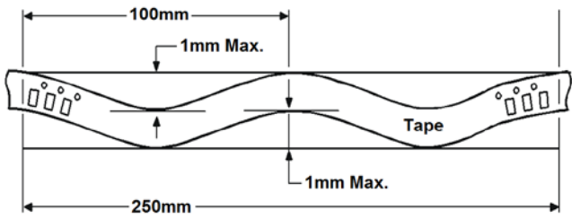
Allowable camber to be 1mm/100mm tape, non-cumulative
