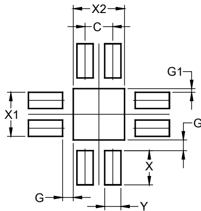
V-QFN3030-8 (Standard)
