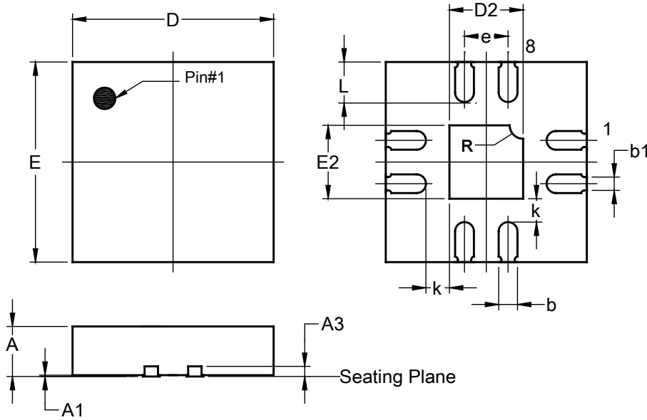
V-QFN3030-8 (Standard)
