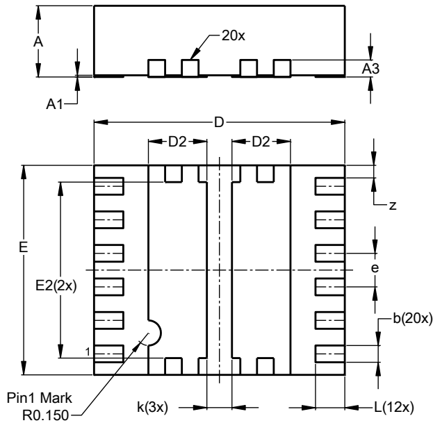
V-QFN3025-20 (Type A)
