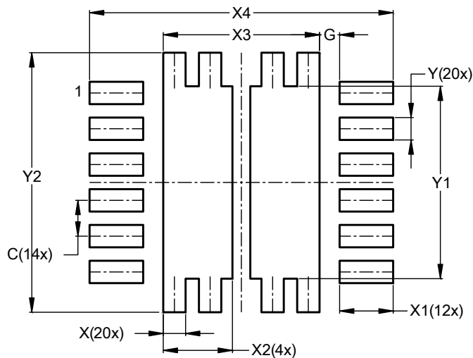
V-QFN3025-20 (Type A)
