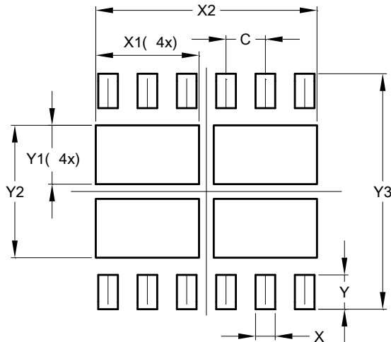
V-DFN5045-12
