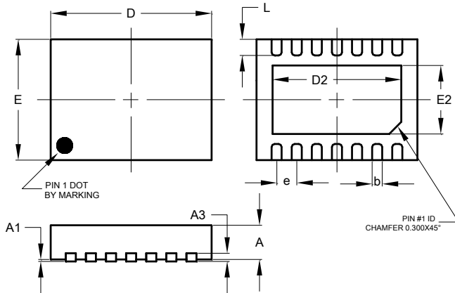
V-DFN4030-14
