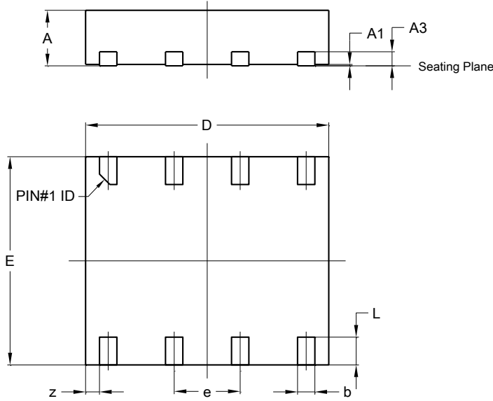
V-DFN3035-8
