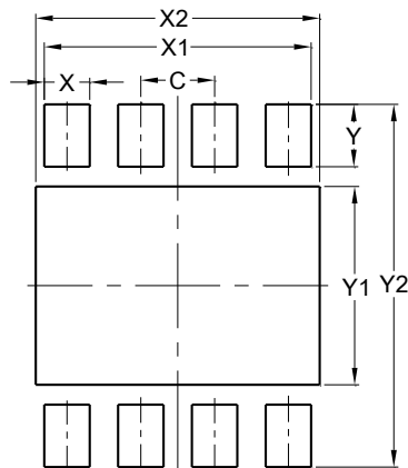
V-DFN3030-8/SWP (Type UX)
