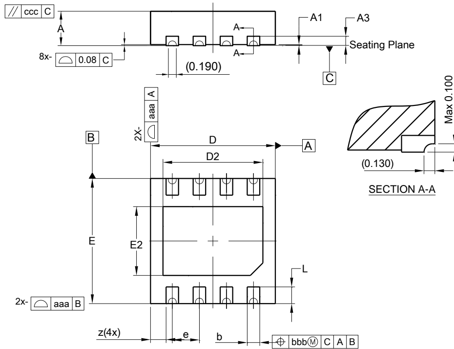
V-DFN3030-8/SWP (Type UX)
