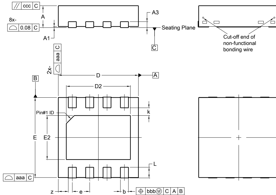
V-DFN3030-8/SWP (Type A)
