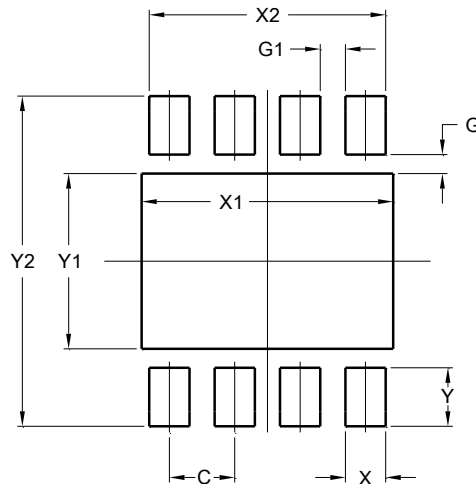
V-DFN3030-8/SWP (Type A)
