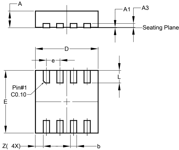
V-DFN3030-8
