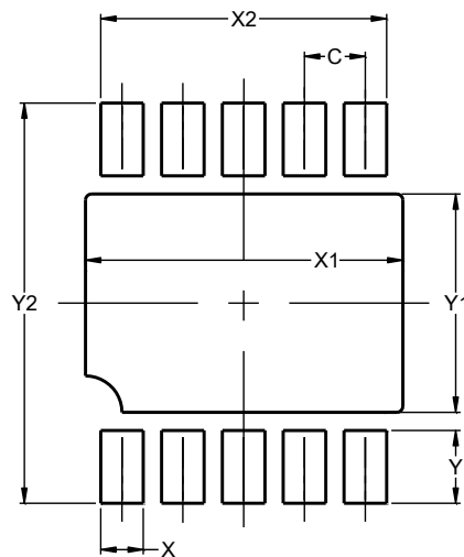
V-DFN3030-10 (Type B)
