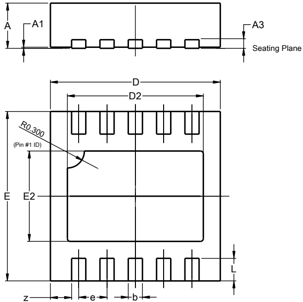
V-DFN3030-10 (Type B)
