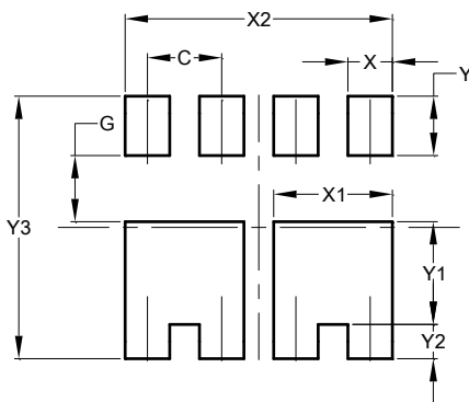
V-DFN3020-8 (Type N)
