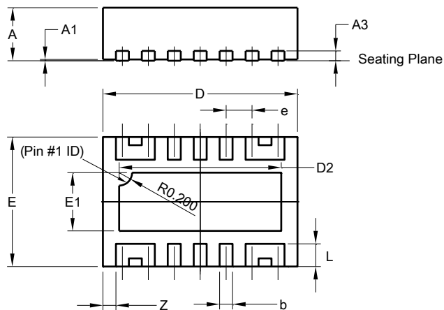
V-DFN3020-14
