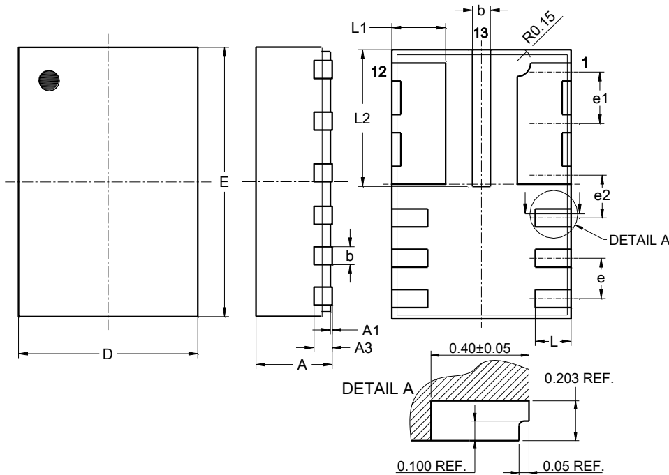
V-DFN3020-13/SWP (Type A1)
