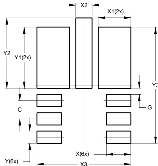
V-DFN3020-13/SWP (Type A1)
