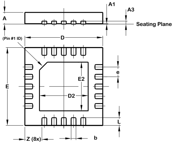
U-QFN4040-20
