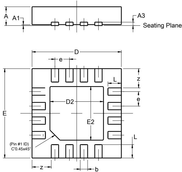
U-QFN4040-16
