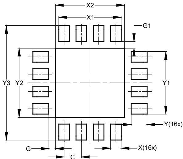
U-QFN4040-16 (Type B)
