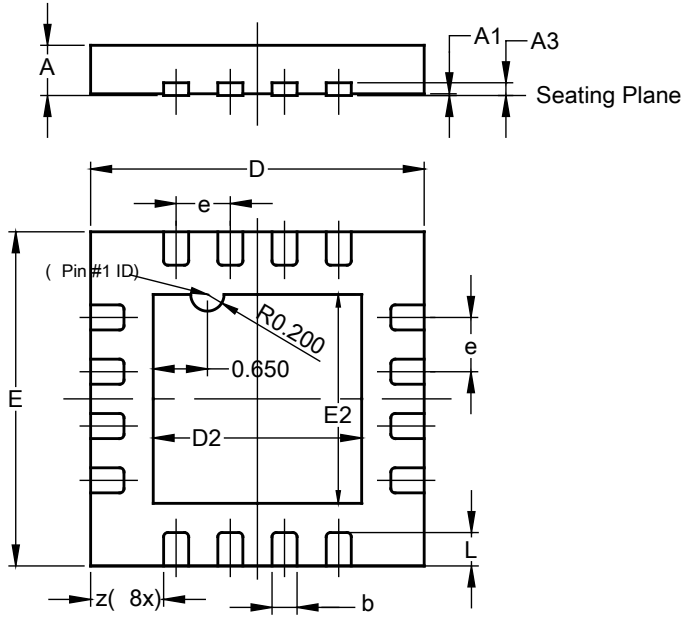
U-QFN4040-16 (Type B)
