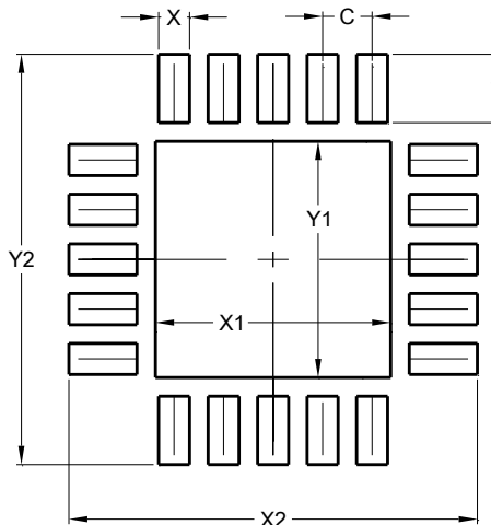
U-QFN3030-20
