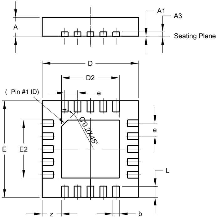
U-QFN3030-20
