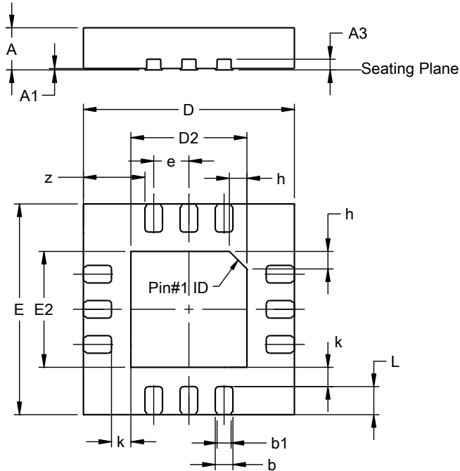
U-QFN3030-12 (Type A)
