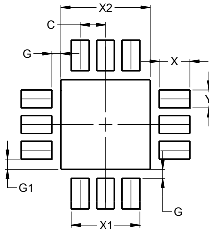
U-QFN3030-12 (Type A)
