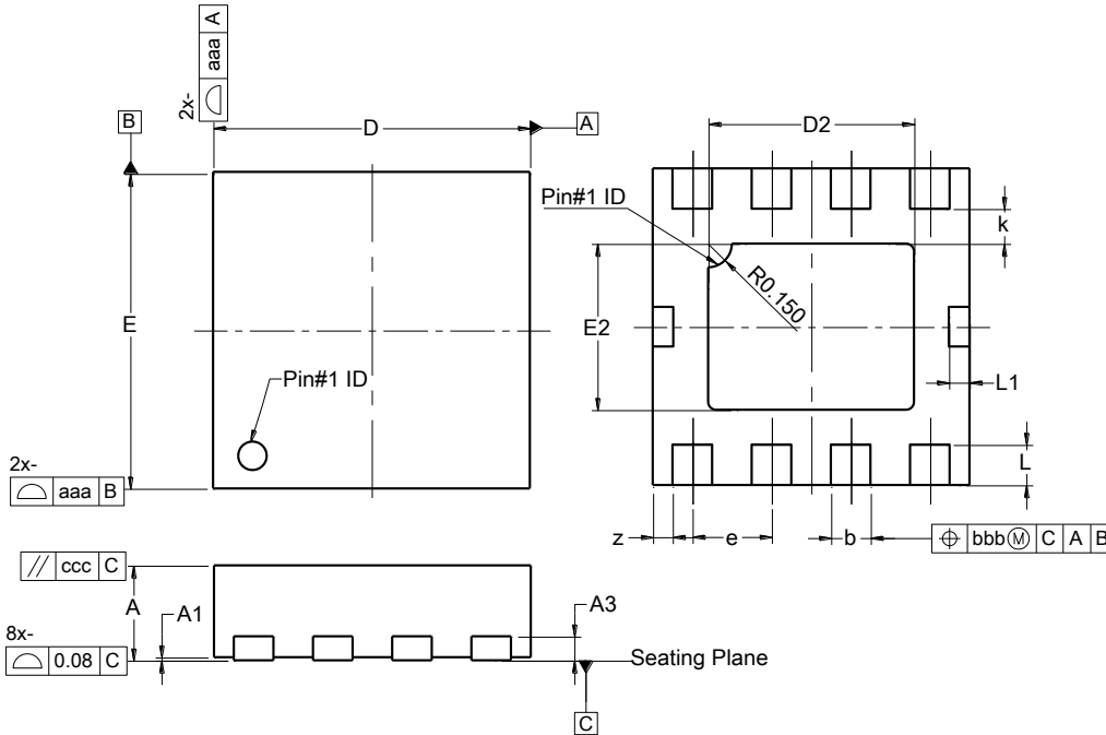
U-QFN2020-10
