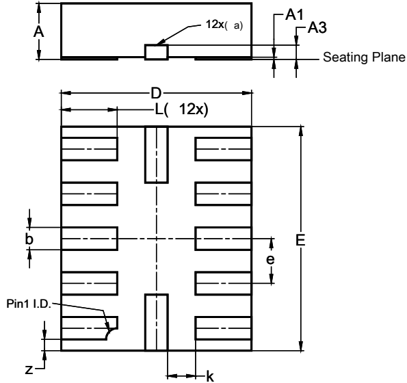
U-QFN1720-12 (Type A)
