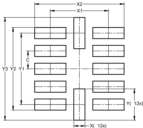
U-QFN1720-12 (Type A)
