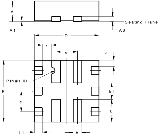
U-QFN1515-10 (Type A)
