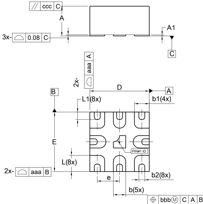
U-QFN1212-9/SWP
