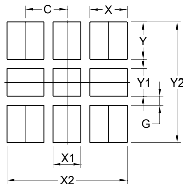
U-QFN1212-9/SWP
