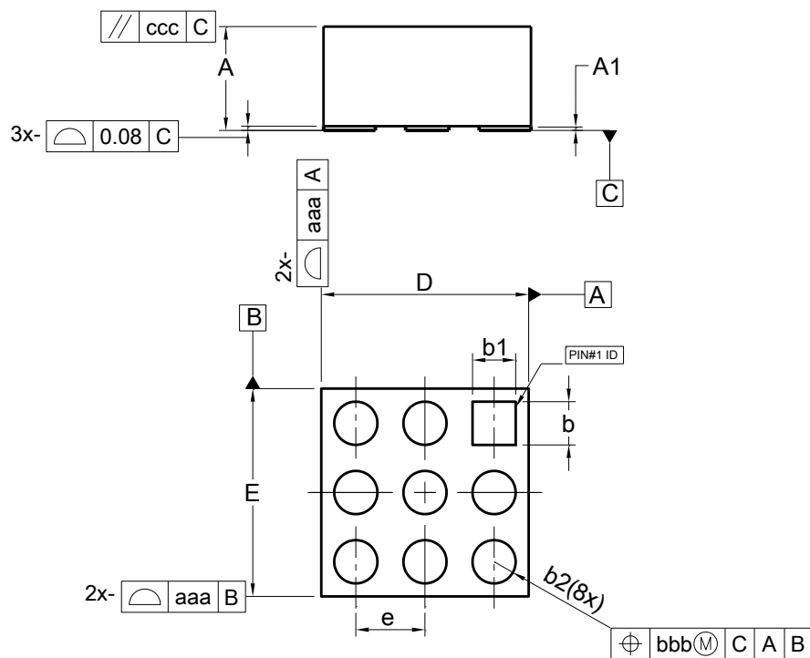
U-QFN1212-9 (Type B)
