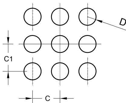
U-QFN1212-9 (Type B)
