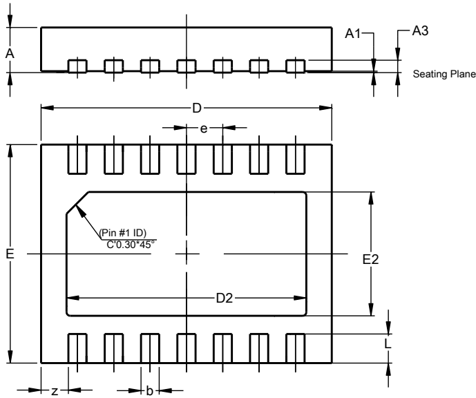
U-DFN4030-14
