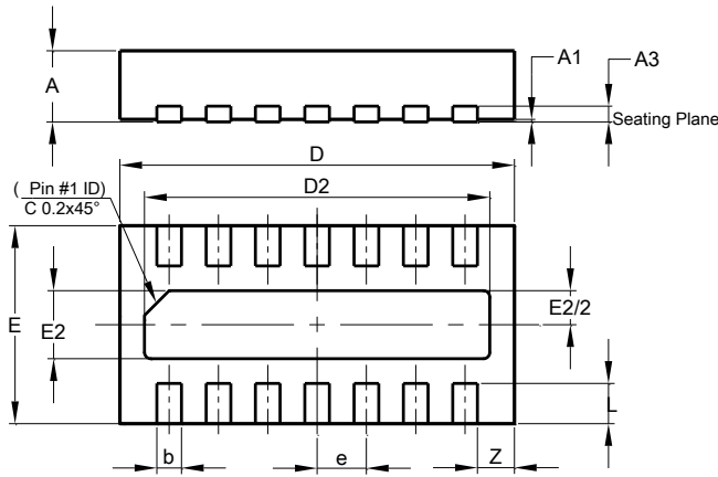
U-DFN3216-14
