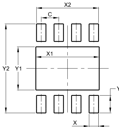
U-DFN3030-8 (Type E)
