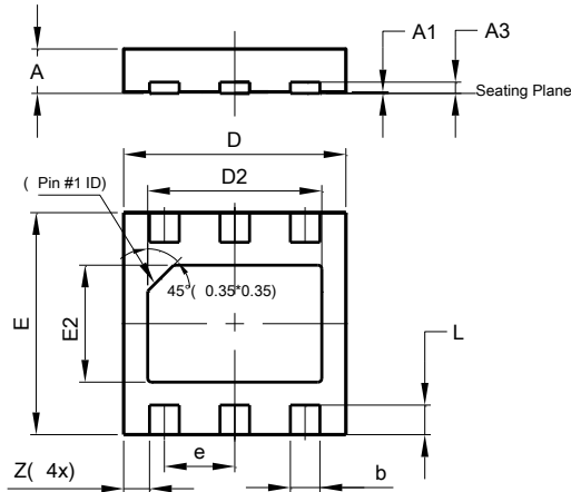
U-DFN3030-6
