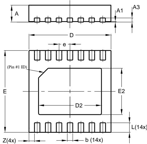
U-DFN3030-14
