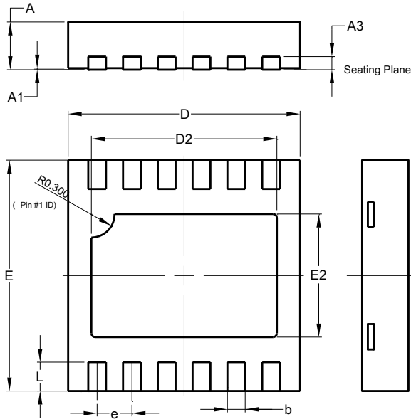
U-DFN3030-12
