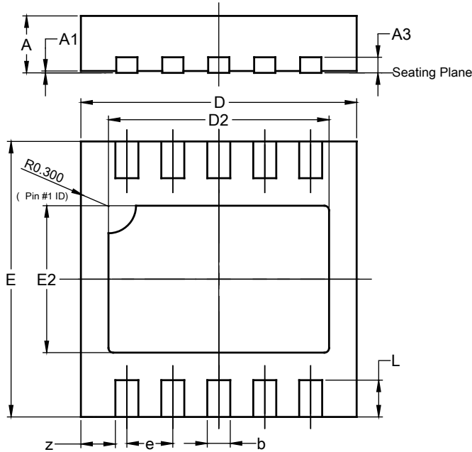
U-DFN3030-10
