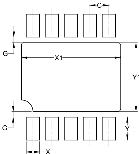
U-DFN3030-10
