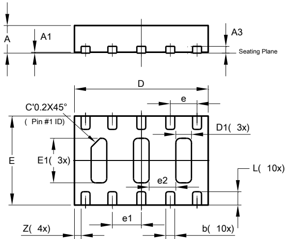
U-DFN3020-10
