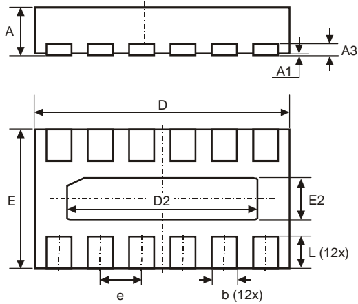
U-DFN3016-12
