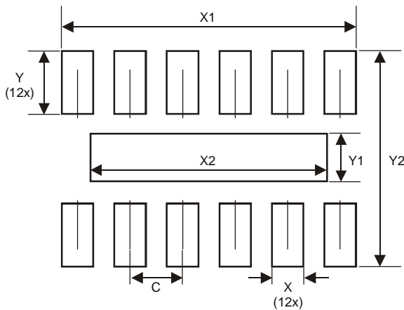
U-DFN3016-12
