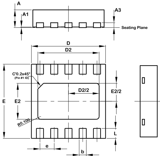
U-DFN2626-10
