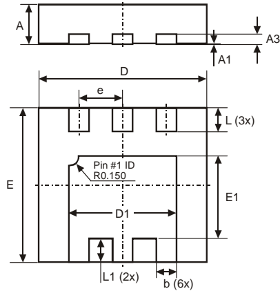
U-DFN2523-6
