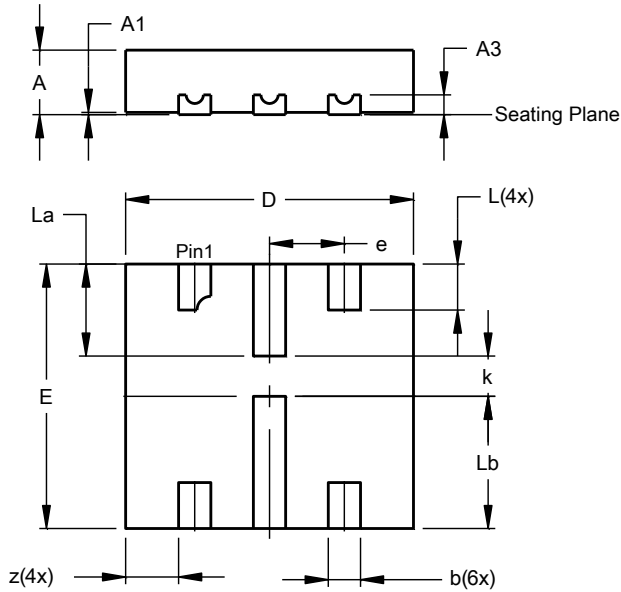
U-DFN2523-6 (Type A)
