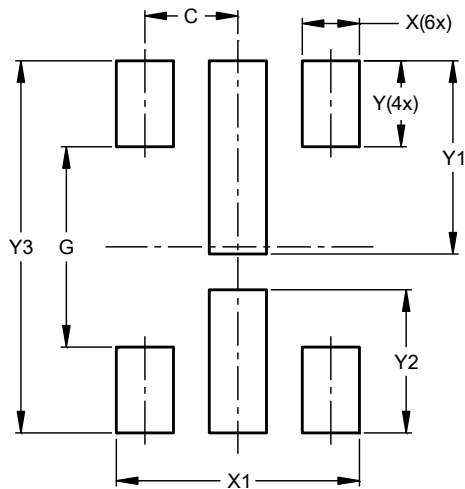
U-DFN2523-6 (Type A)
