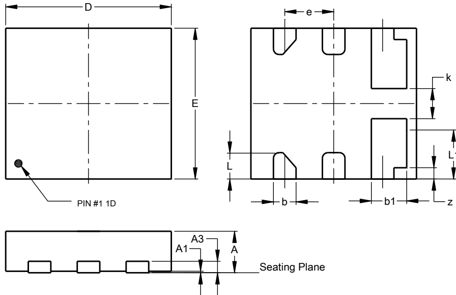
U-DFN2220-6 (Type A1)
