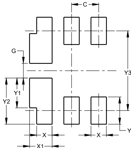
U-DFN2220-6 (Type A1)
