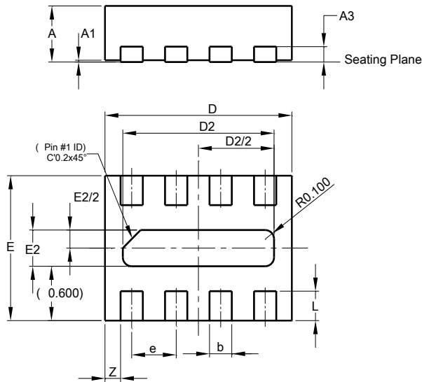
U-DFN2116-8
