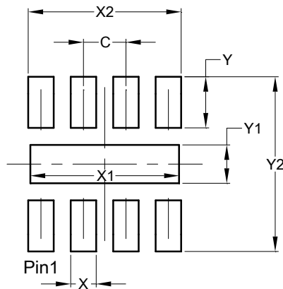
U-DFN2116-8
