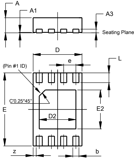
U-DFN2030-8
