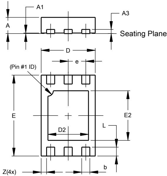
U-DFN2030-6
