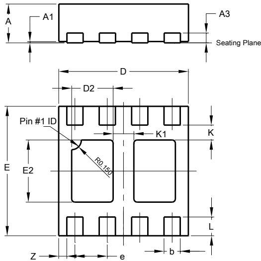
U-DFN2020-8
