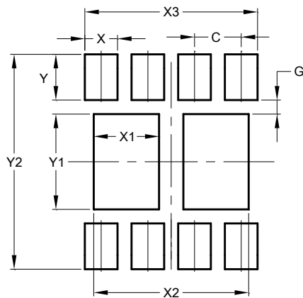
U-DFN2020-8
