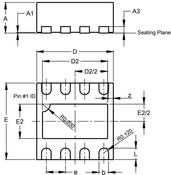
U-DFN2020-8 (Type E)
