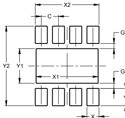
U-DFN2020-8 (Type E)
