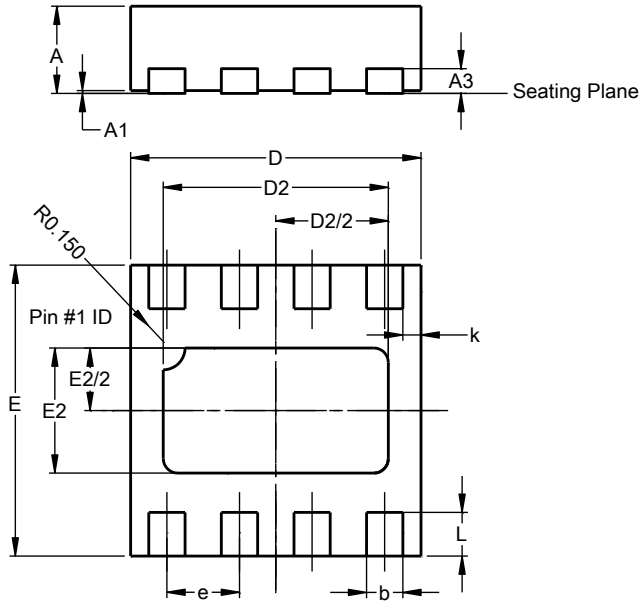
U-DFN2020-8 (Type A)
