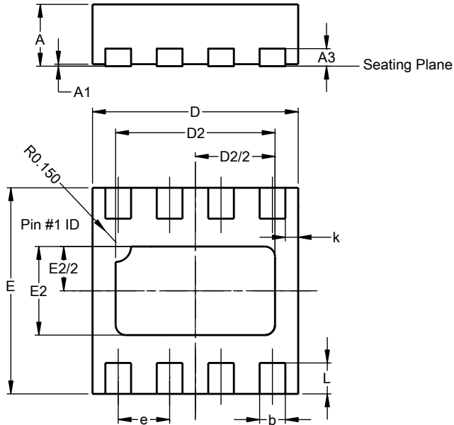
U-DFN2020-8 (Type A)
