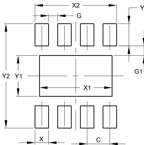
U-DFN2020-8 (Type A)
