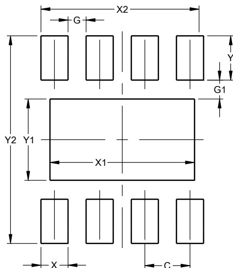
U-DFN2020-8 (Type A)
