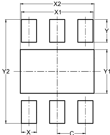
U-DFN2020-6 (SWP) (Type UXC)
