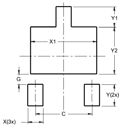
U-DFN2020-3 (Type B)
